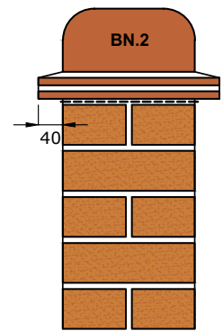
Creasing tiles and double bullnose to form coping
