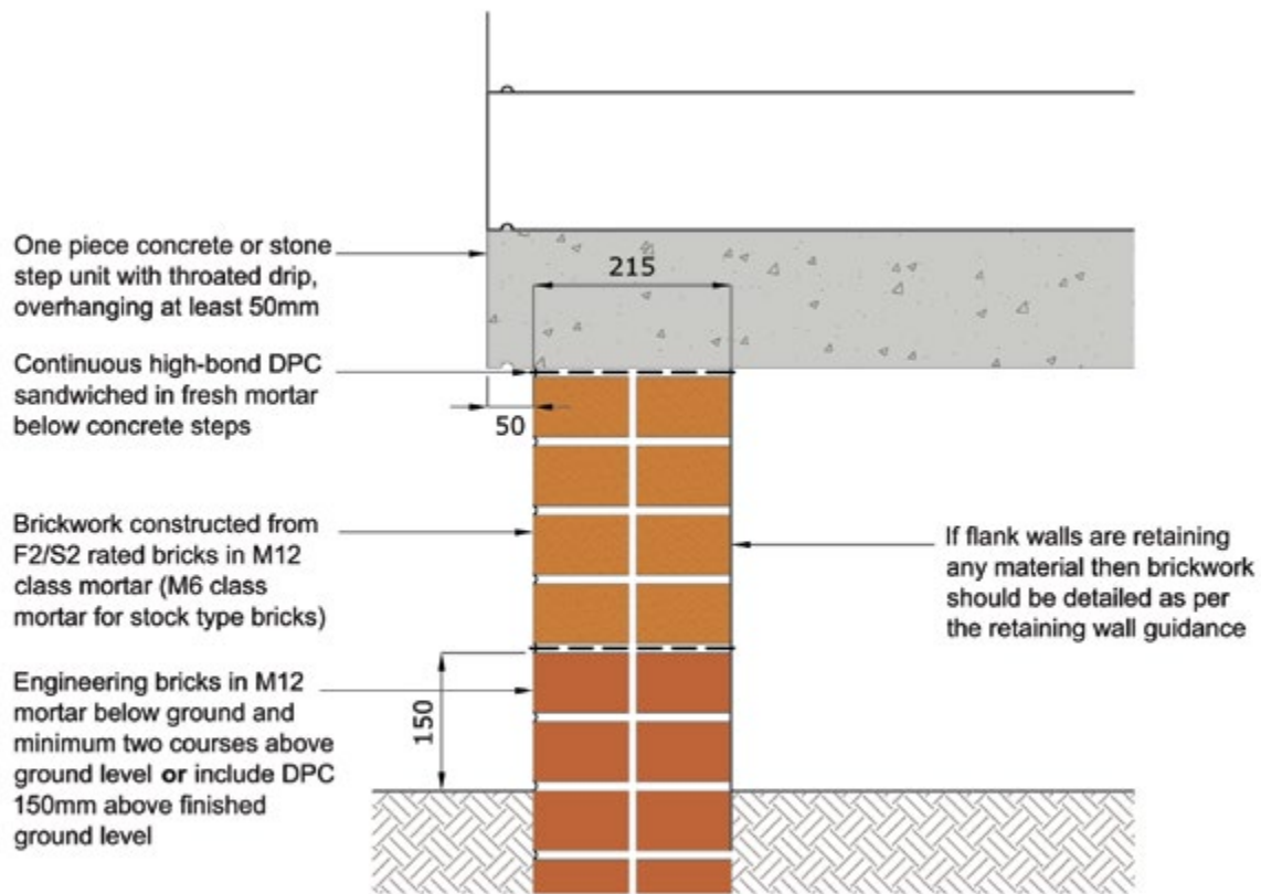
Step Flank Walls Cross Section
